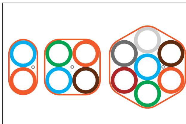
Microduct Bundles 12/8mm.
