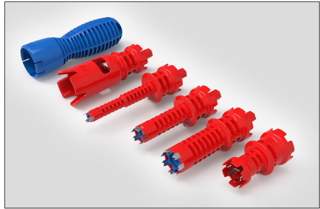
Port Opening Tool Sizes B/S, SD, RD, BD and ST
